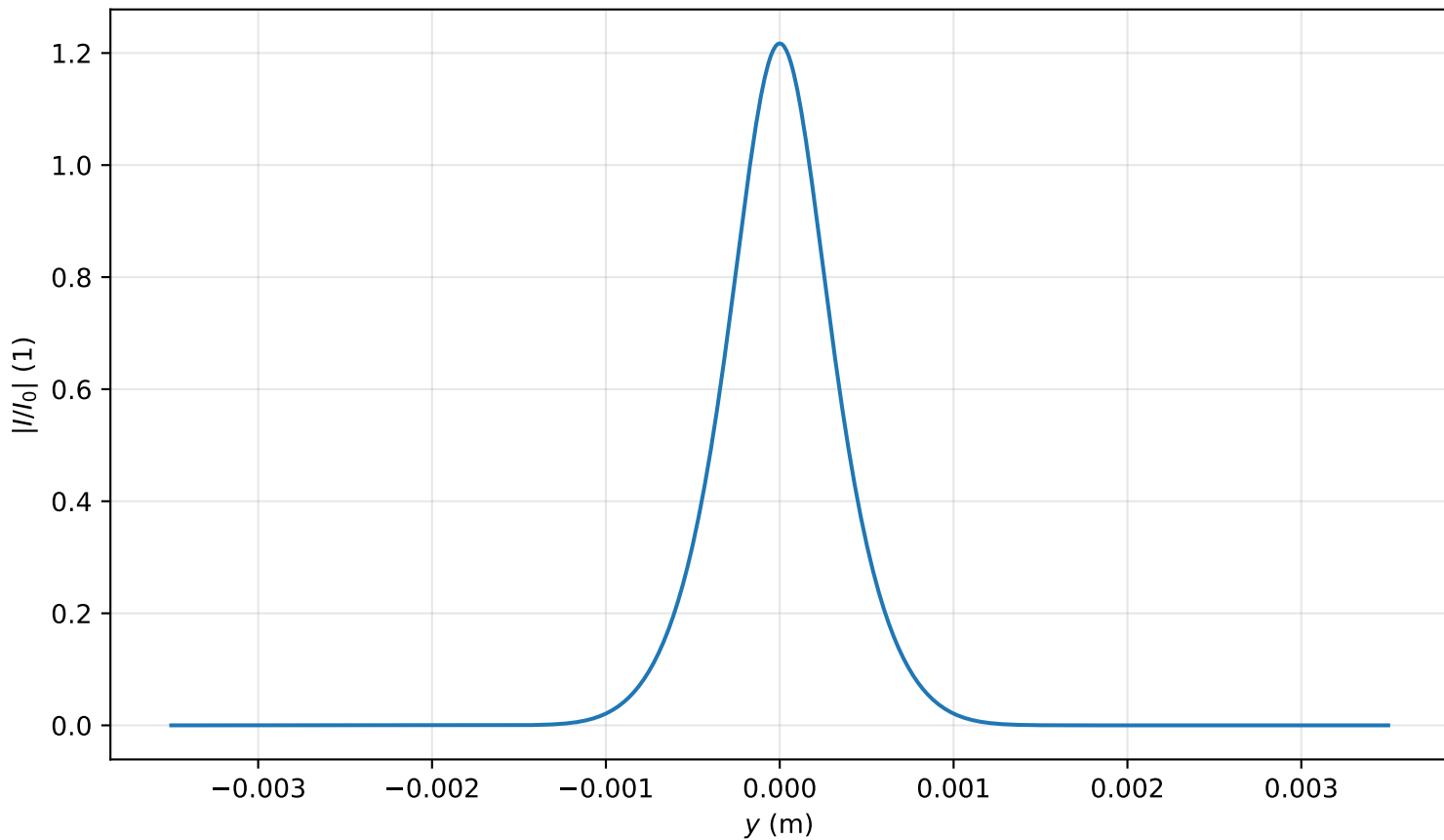
Intensity profile I(x=0, y, z=0.637)/I_0 , P_{in}=0.9P_{cr} , artificial time
